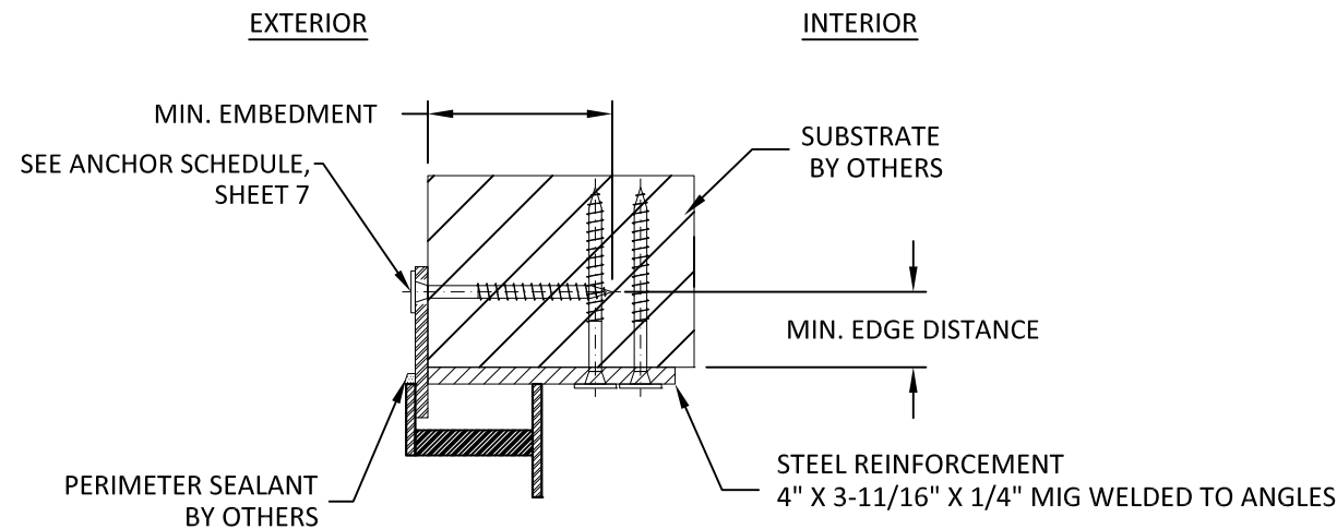
J 9 VERTICAL SECTION HEAD - INTERIOR NAIL FIN CLIP
