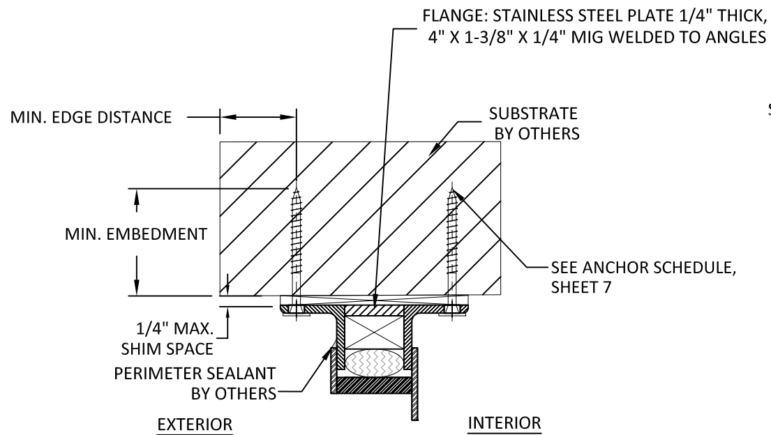
H 9 VERTICAL SECTION HEAD - EXTERIOR ANGLE FLANGE CLIP
